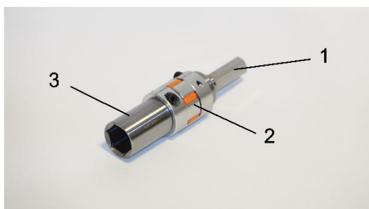
Complete Drive Unit
